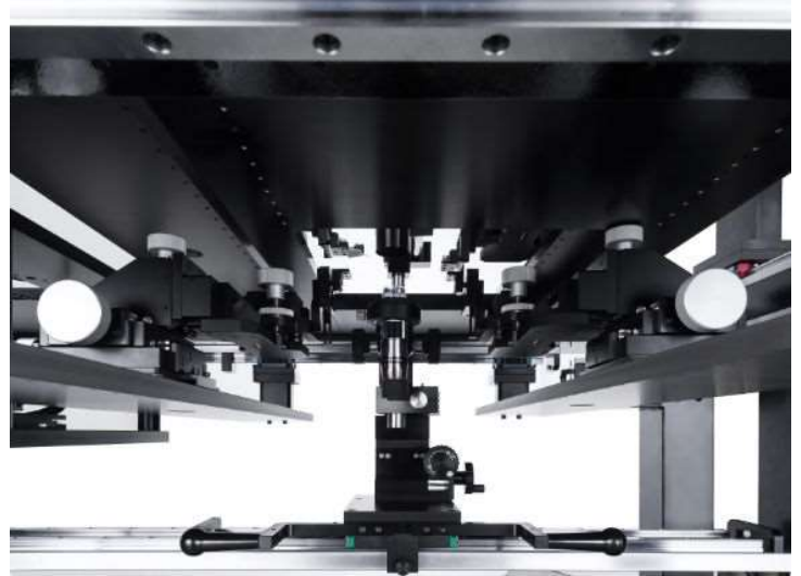
PCB probe station for use with mmW capability with double side probing feature (open section for sample)
